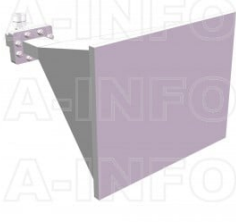
LB-137-20-C-7SPO Standard Gain Horn Antenna 5.85-8.2GHz 20dB Gain 7mm
